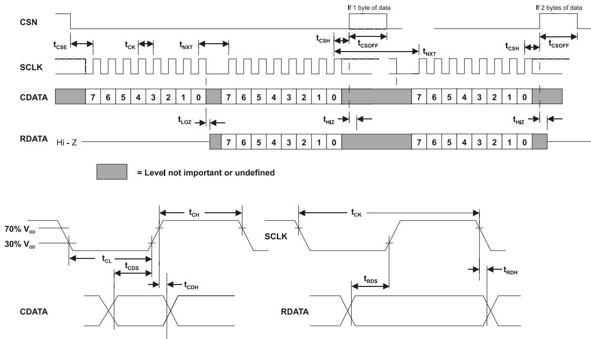
Figure 27 C-BUS Timing
